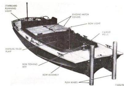
Figure 1-1. 27-foot bridge erection boat, right front view.
